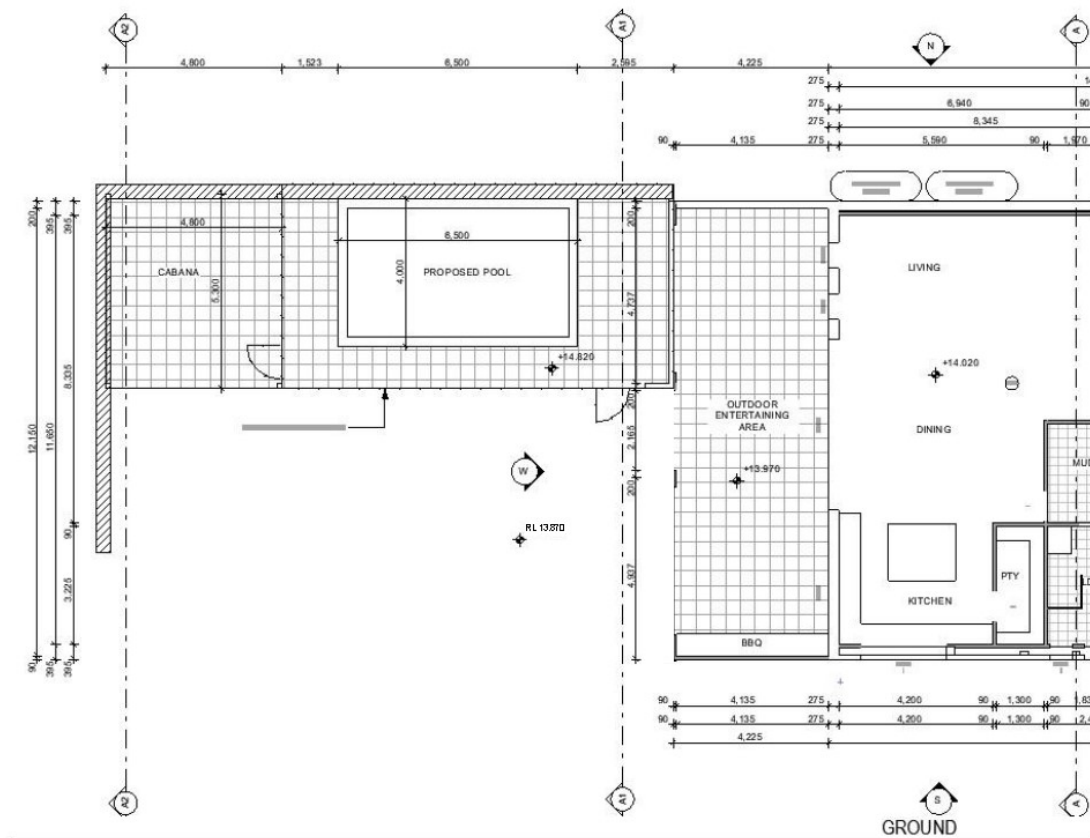
GROUND FLOOR/ PART WITH SECTIONS A1 & A2
