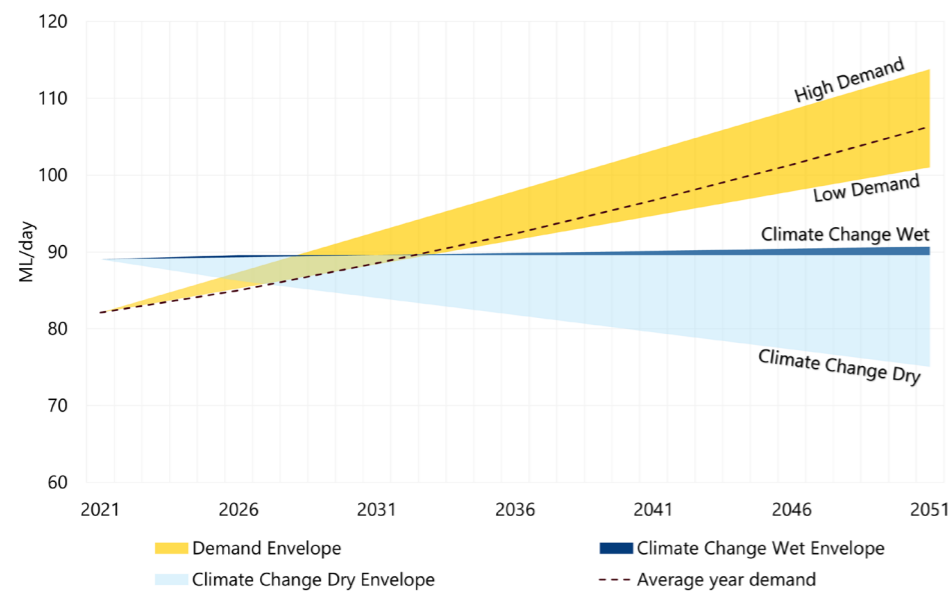
Figure 14: Supply and demand forecasts with boundaries of uncertainty (note the y axis starts at 60 ML/d)
