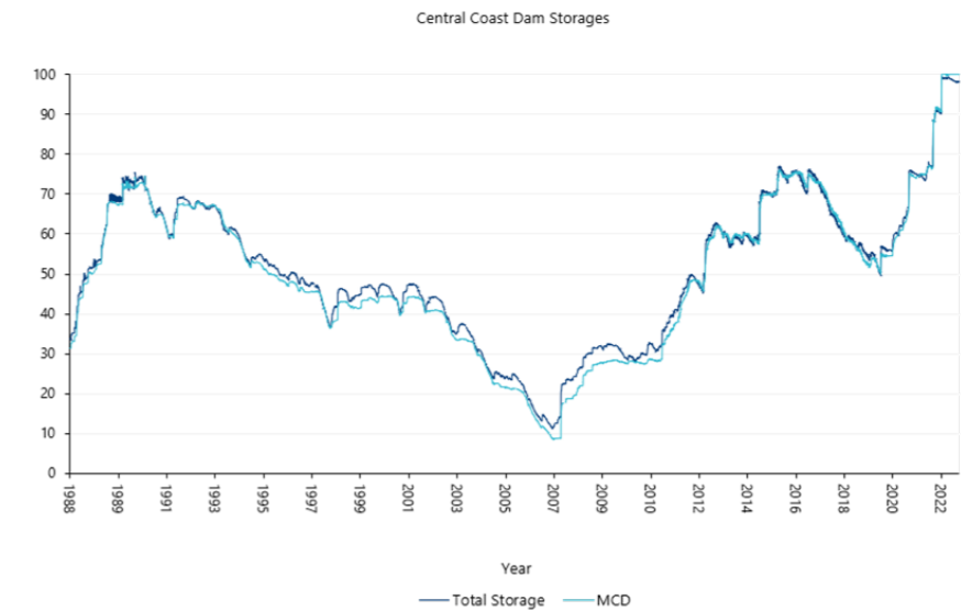
Figure 9: Historical storage level in Mangrove Creek Dam (MCD)
