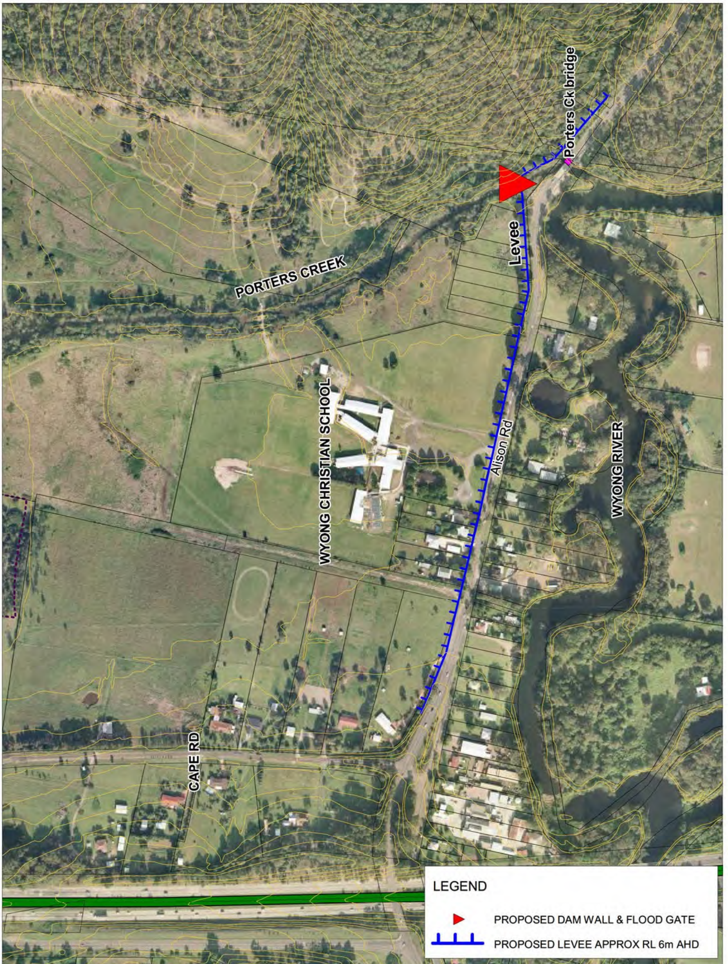
FIGURE 11.1 Structural Option 1.1
