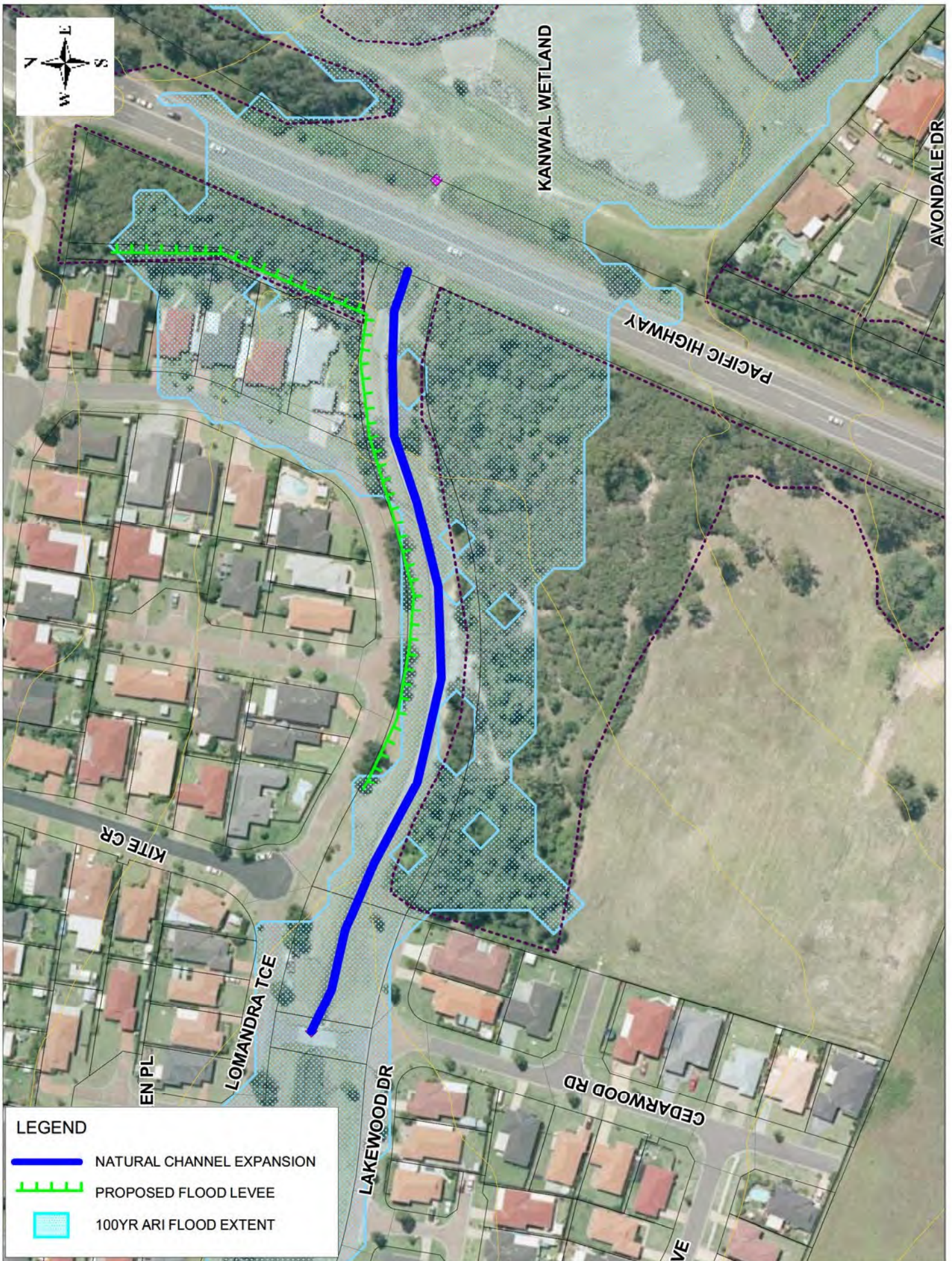
FIGURE 11.4 Structural Option 1.4
