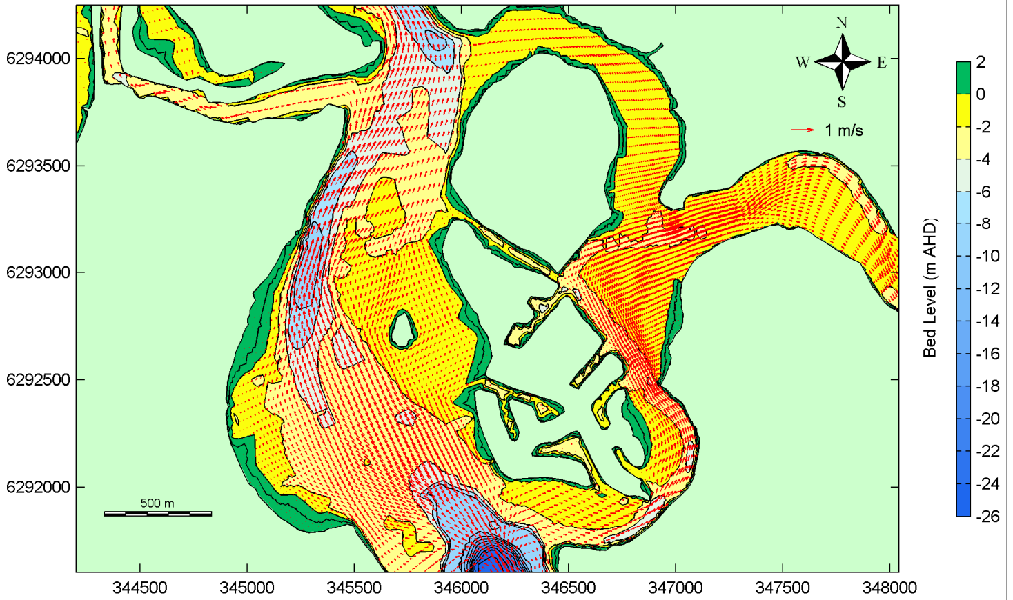
Flood Tide 10:00 07/04/2004
