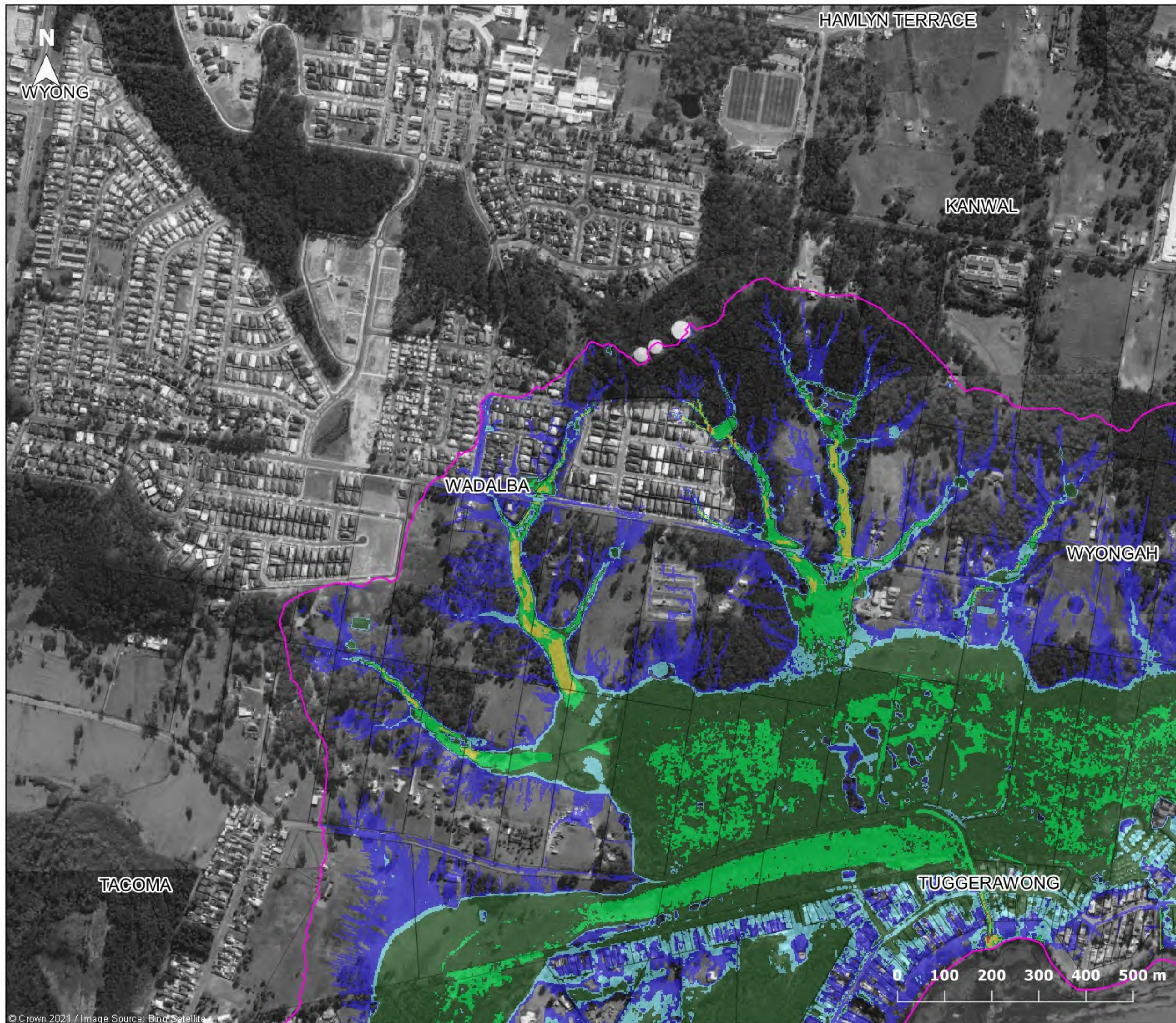
Figure D2.2 Probable Maximum Flood Life Hazard Categories
