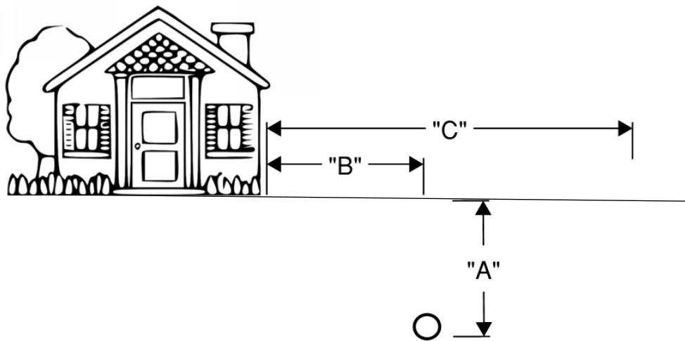
Figure 1 Required clearances and corridor to avoid replacement of AC/CI/VC gravity sewer mains at the time of development
