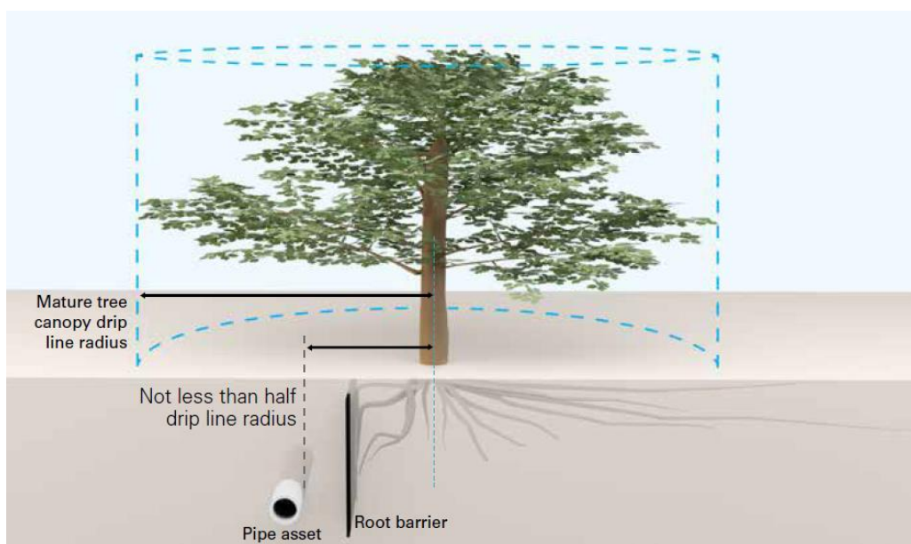
Figure 7 Recommended measures if planting trees in the vicinity of Council pipelines (courtesy of SWC)
