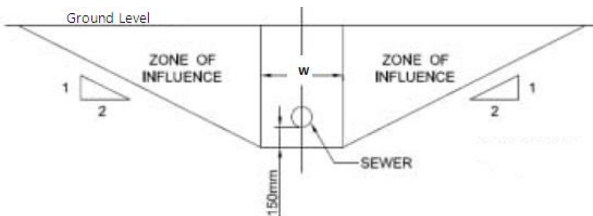
Figure 2 Zone of Influence Diagram
