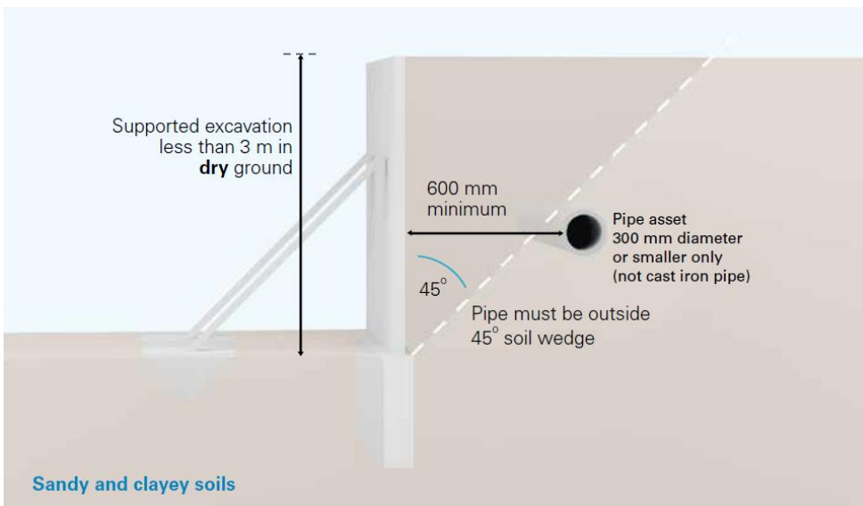
Figure 6 Requirements for small supported excavations (courtesy of SWC)
