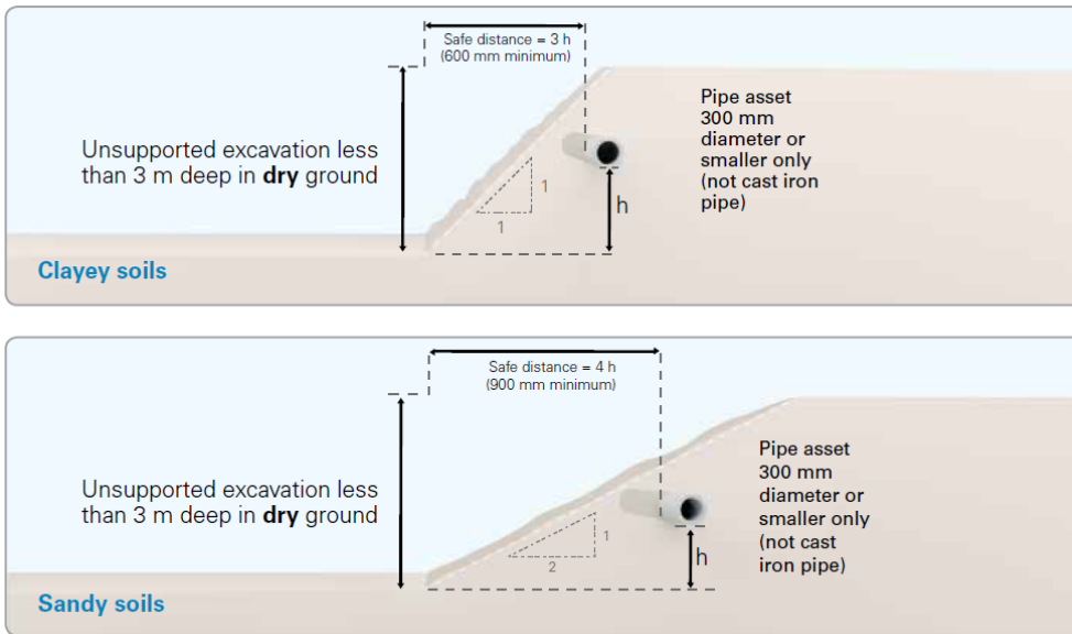
Figure 5 Requirements for small unsupported excavations (courtesy of SWC)
