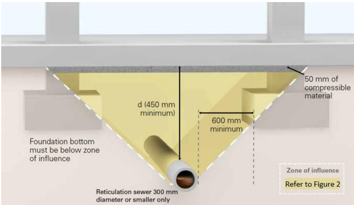
Figure 3 Clearance requirements for foundations in proximity to gravity sewer mains (courtesy of SWC). Note extent of Zone of Influence calculation provided in Figure 2.
