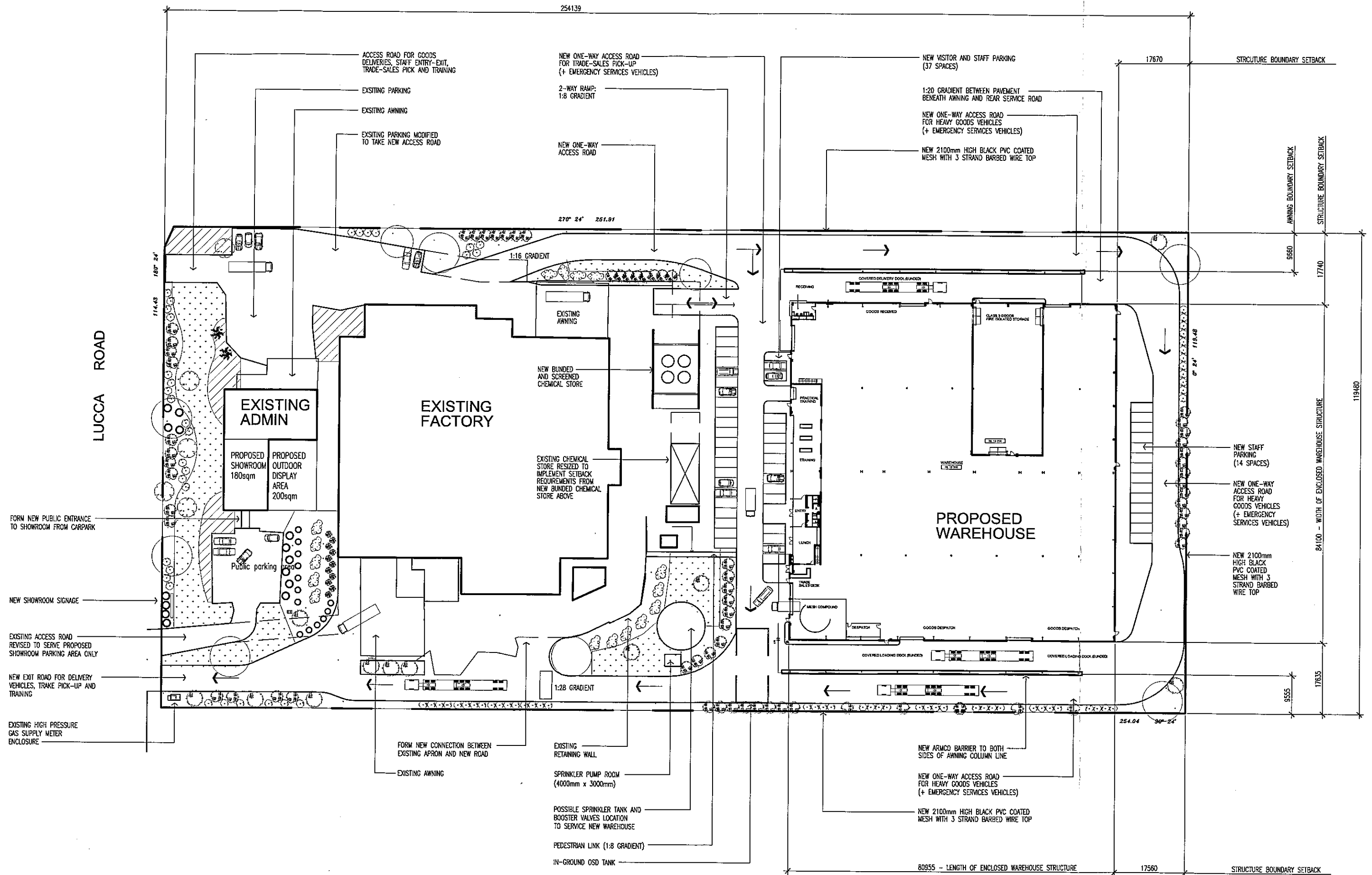
Figure 4 : Site Layout
