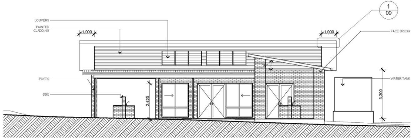
1 06 Elevation - Camp Kitchen Scale: 1 : 100 Notes:
