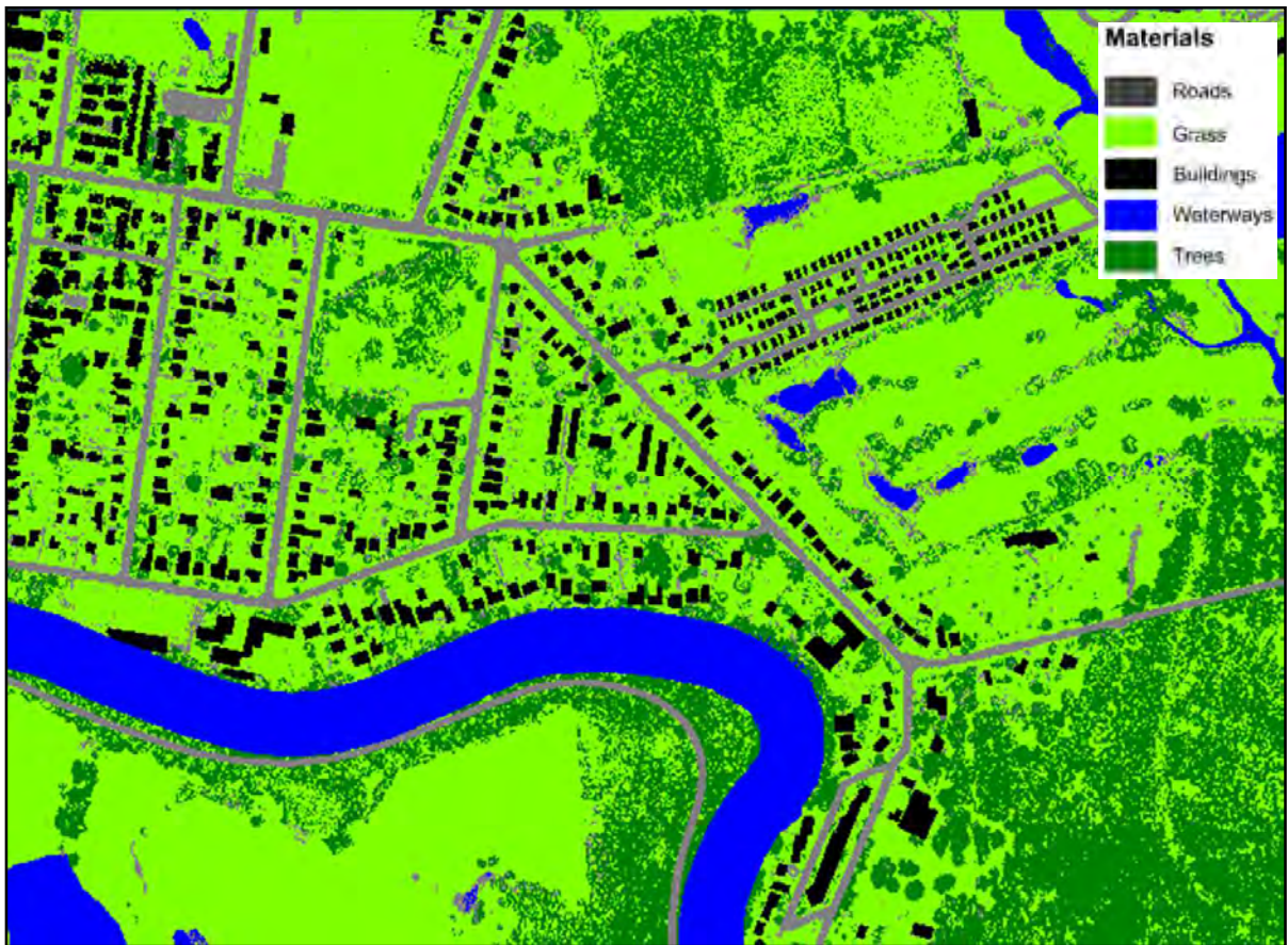
Plate 1 Example of remote sensing output (bottom image) and aerial image (top image) for a section of Wyong
